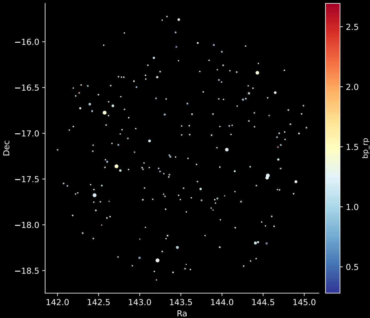
APOGEE DR17 Field: [200-60] Stars: 211
