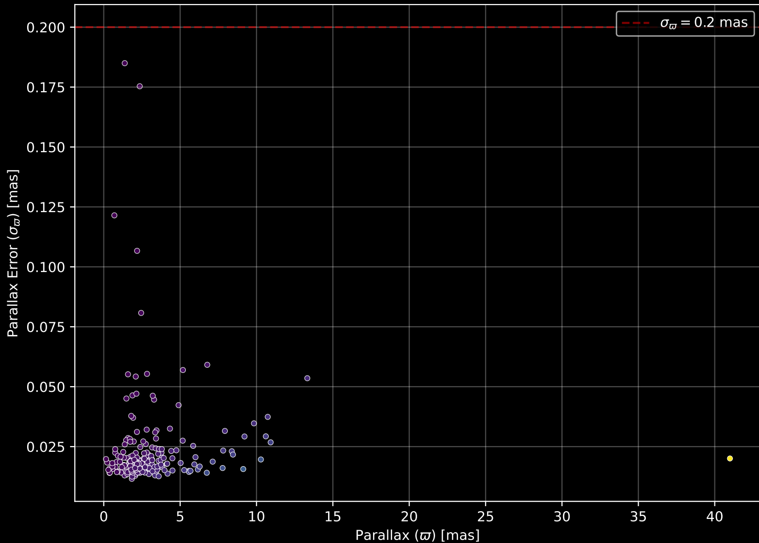
APOGEE DR17 Field: [200-60] Parallax Quality (n= 211)
