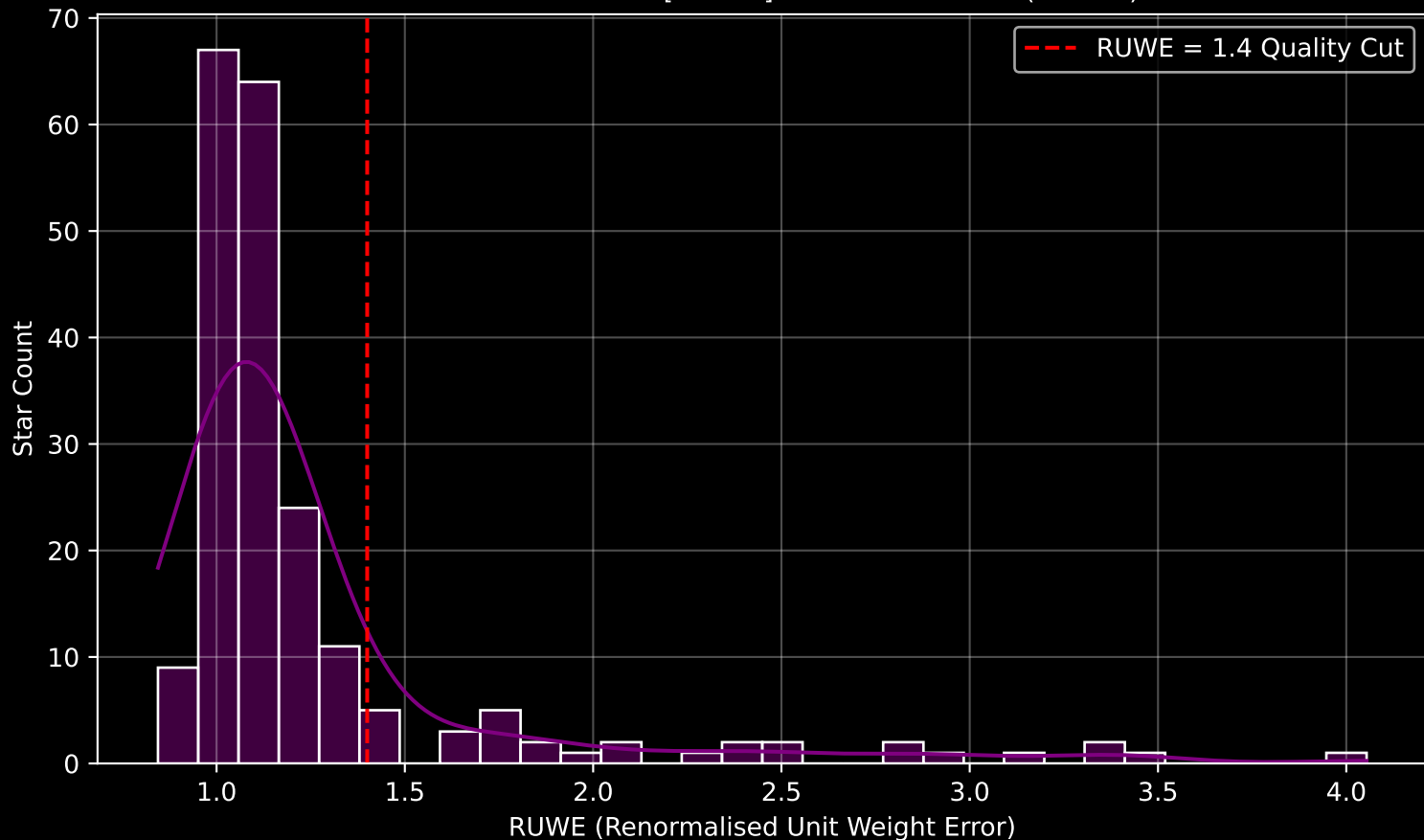
GAPOGEE DR17 Field [200-60] RUWE Distribution (n= 206)
