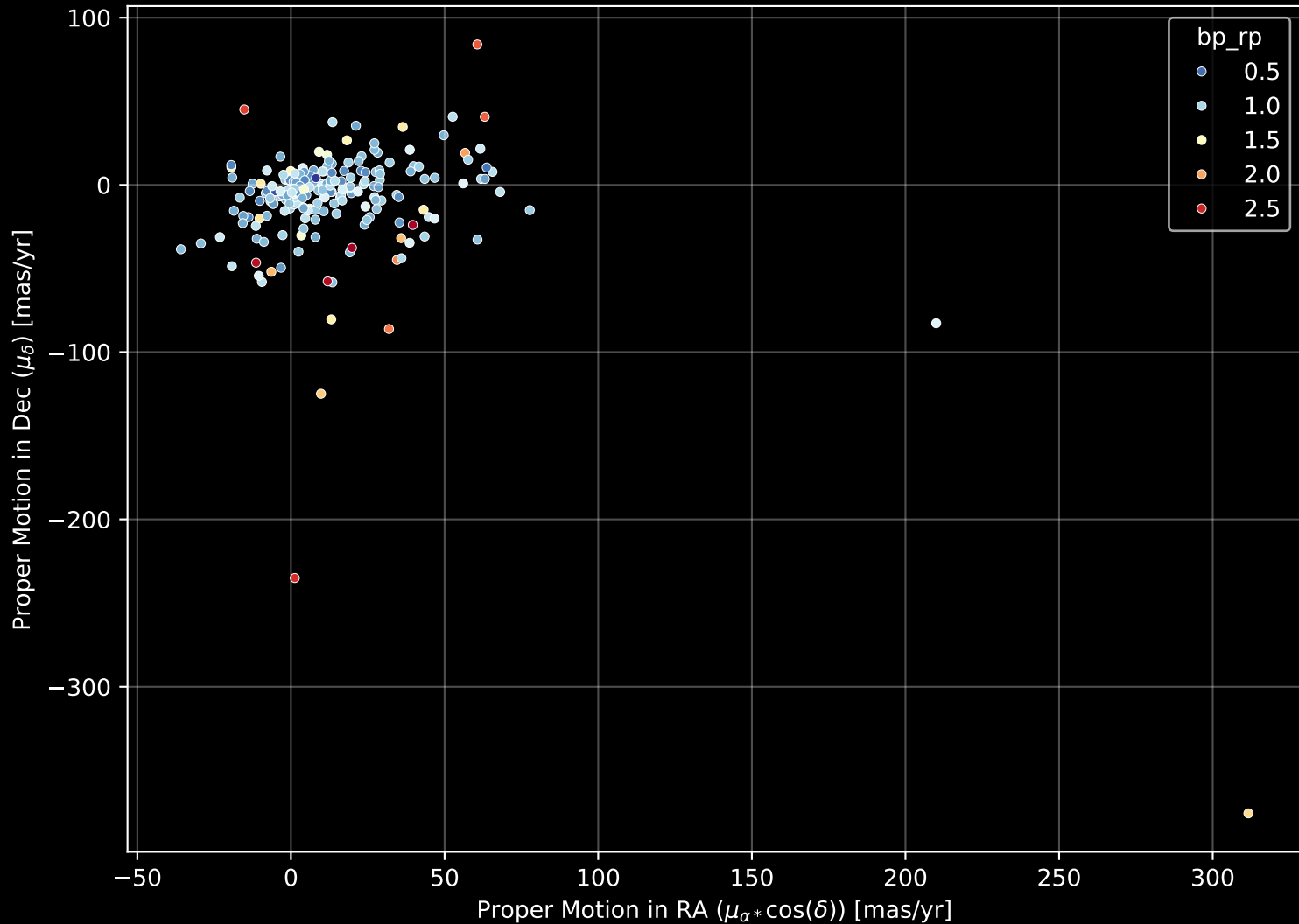
APOGEE DR17 Field: [200-60] Proper Motion Diagram (n= 211)
