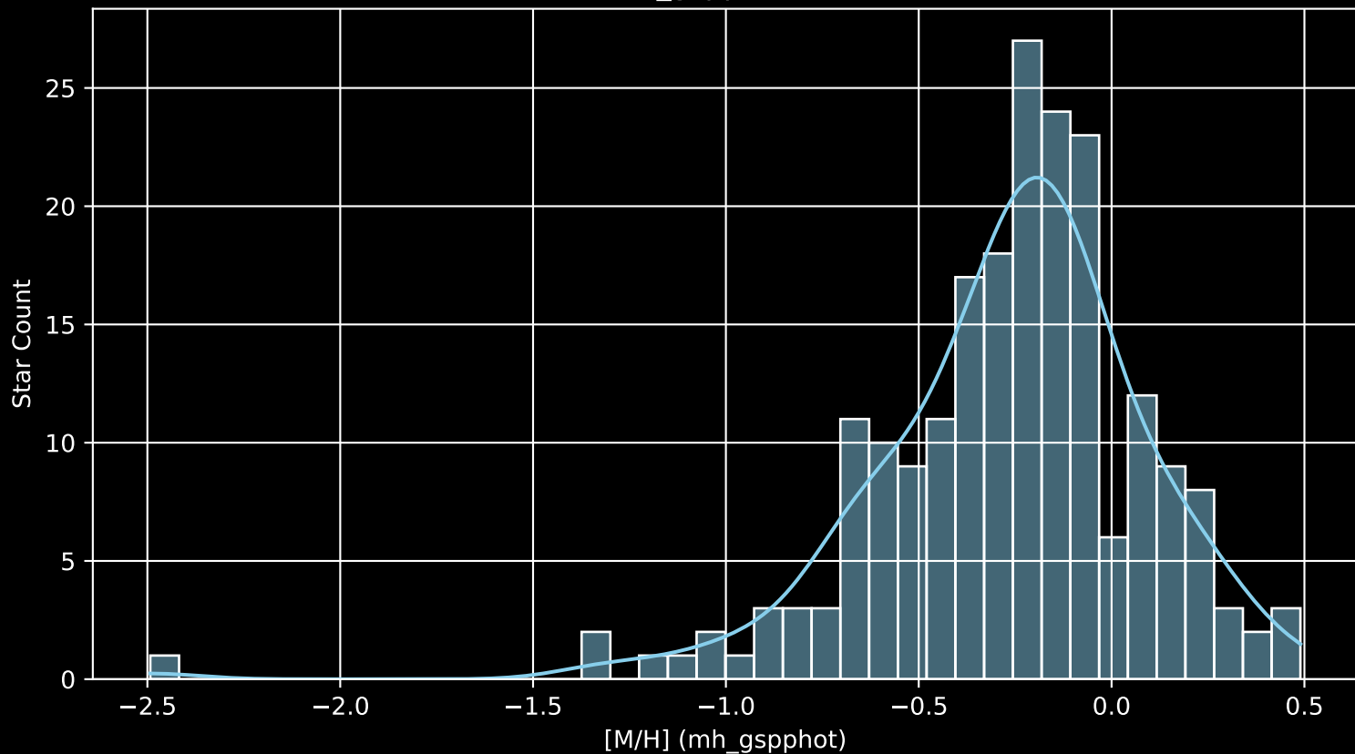
APOGEE DR17 Field: [200-60 [M/H] (mh_gspphot) (n= 210)
