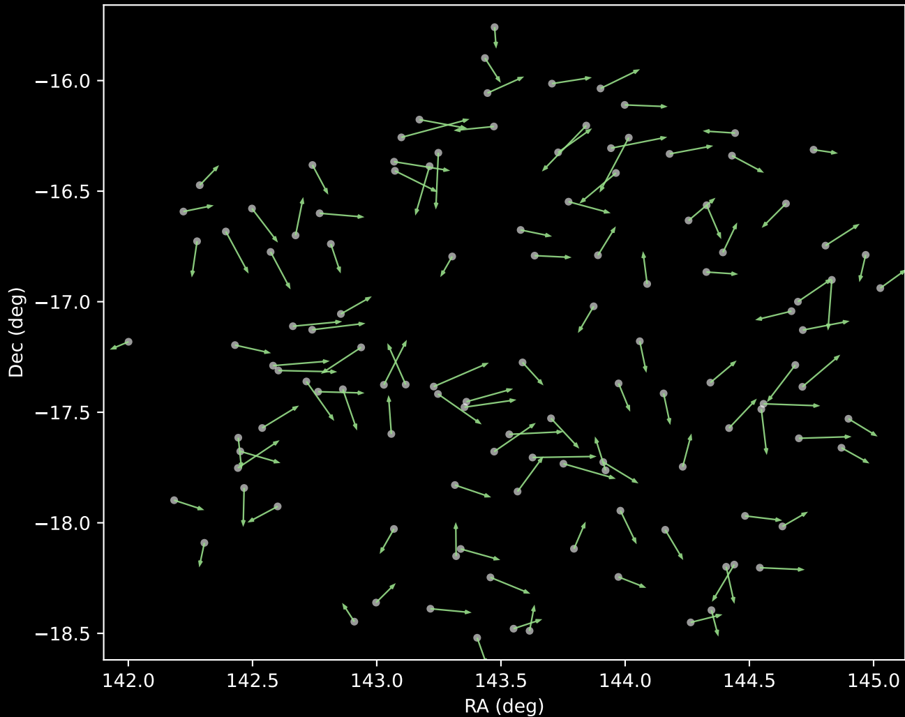
APOGEE DR17 Cluster 5 Proper Motion Vectors (n=121)
